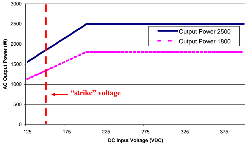
Fig. 11 AC Output power of PVI 1800/PVI 2500
