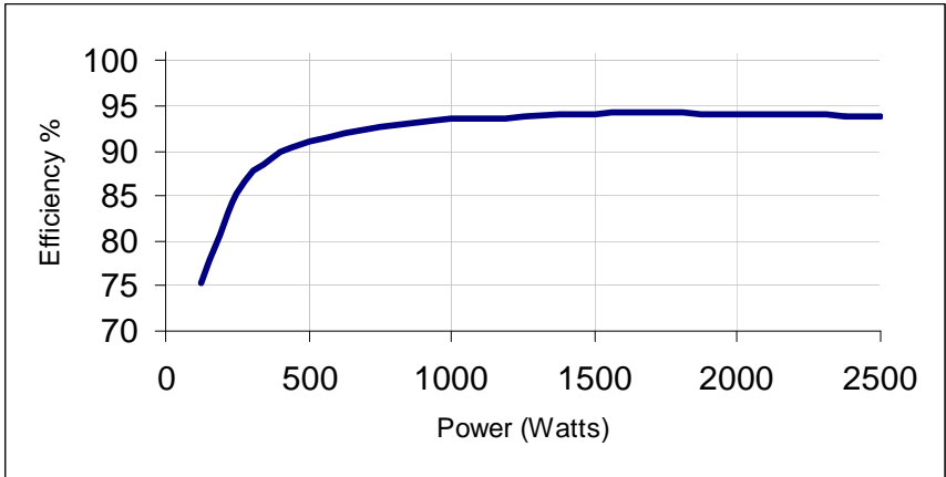
Fig. 13b PVI 2500 efficiency plot
