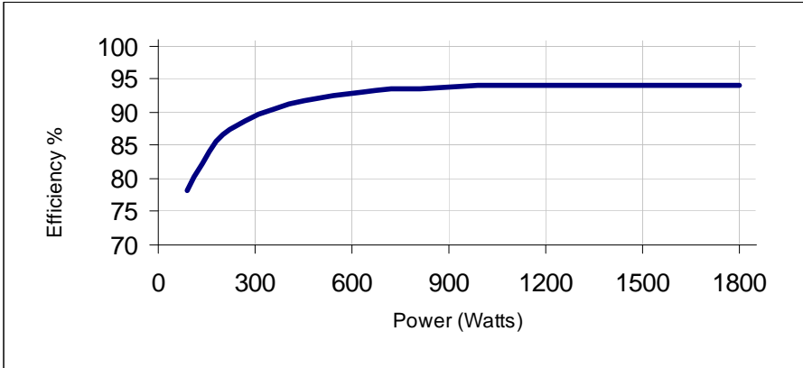
Fig. 13a PVI 1800 efficiency plot
