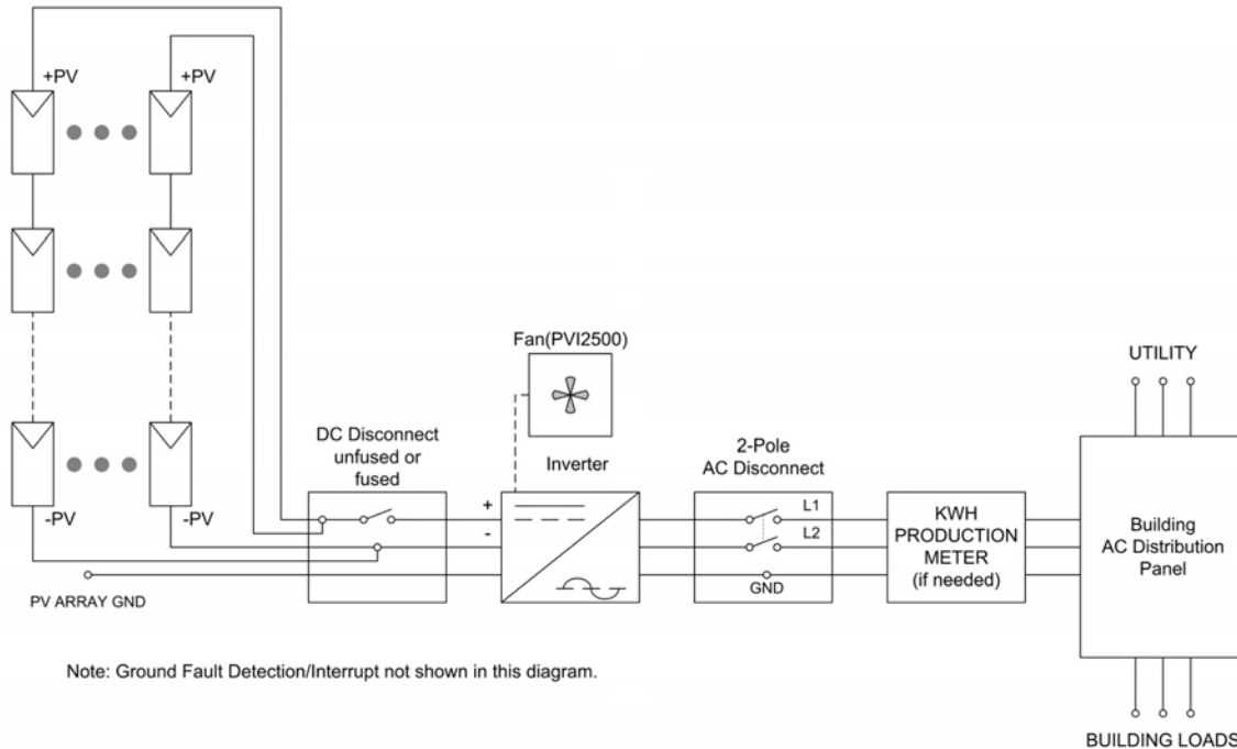
Fig. 6 Simplified electrical connection diagram
