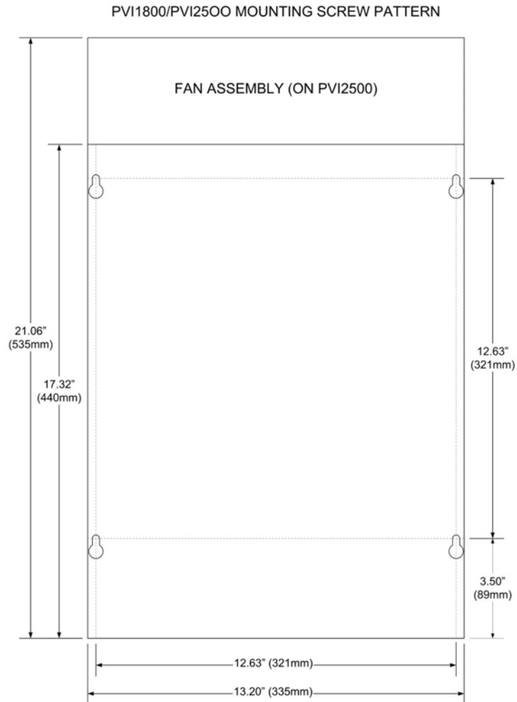
Fig. 5 PVI 1800/PVI 2500 Mounting Screw Pattern
