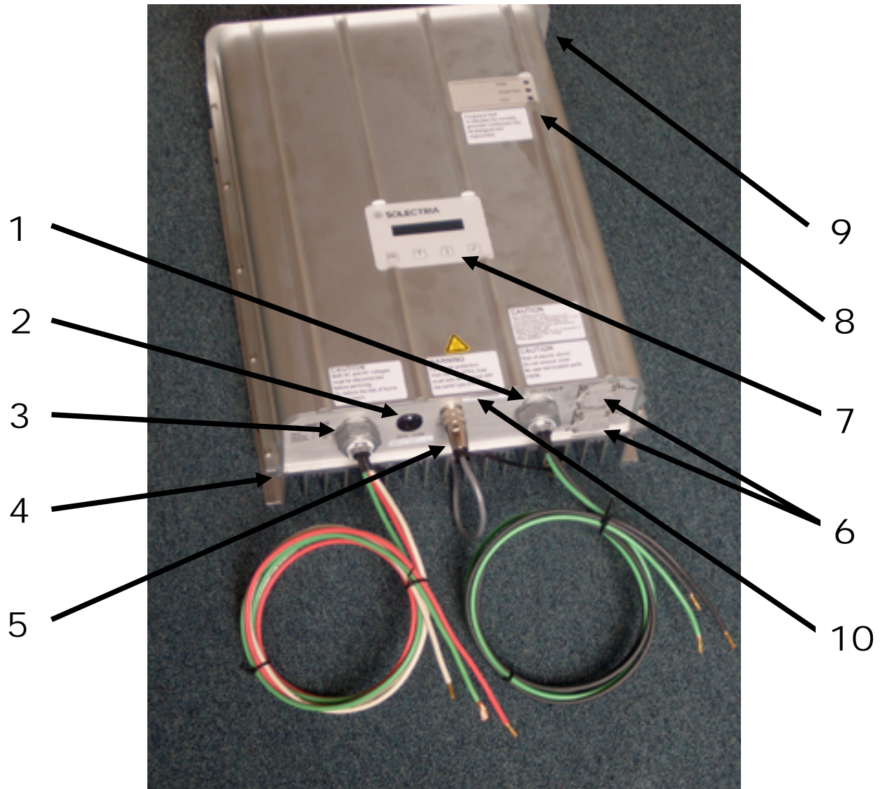
Fig. 2 PVI 1800/PVI 2500 Features Diagram
