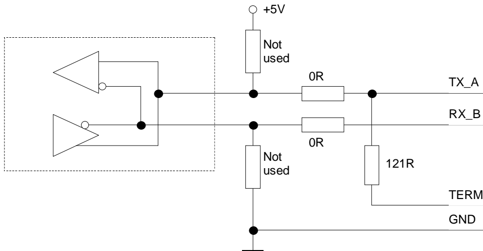
Representative RS485 schematic, inside the inverter
